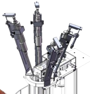
2 PILOTED INJECTORS
